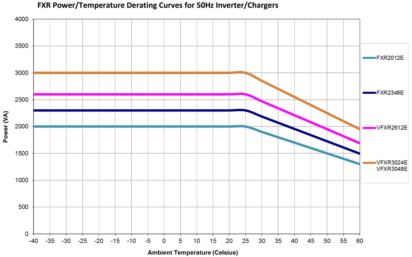
Figure 2: Power/Temperature de-rating for FXR 50Hz models
